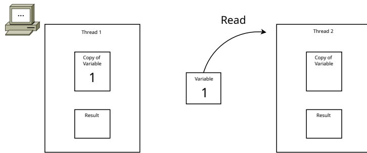
Figure 116: While Thread 1 is working, Thread 2 reads the variable
